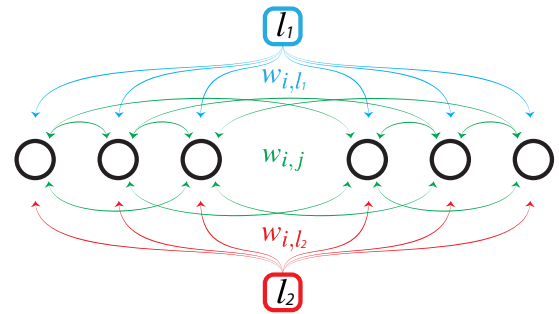
Figure 4: Graph Construction. Stroke segments are shown as black circles. Terminal labels (in this example l_1 and l_2 ) are shown as colored squares. The graph edges w_{i,j} reflect the smoothness terms V_{i,j} between the stroke segments i, j \in S , while the data terms D_i(l) for stroke segment i \in S and label l \in L are captured by the weights w_{i,l} .
